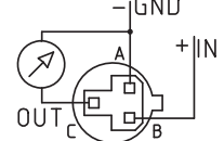
B (IN) C (OUT) A (GND)
