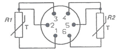
Pin assignment 2xPt100
